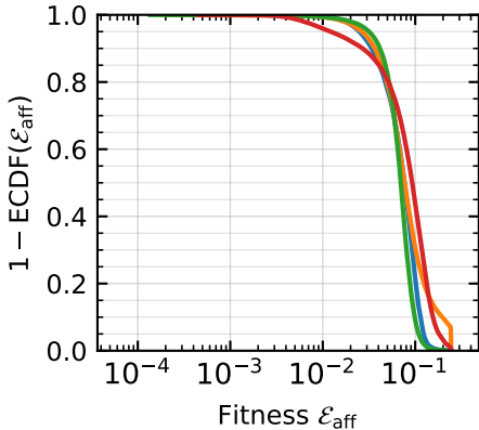
ReLU
