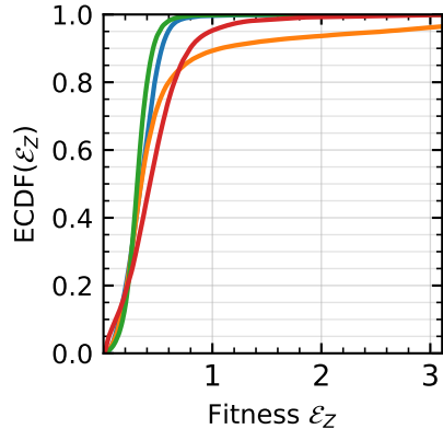
ReLU
