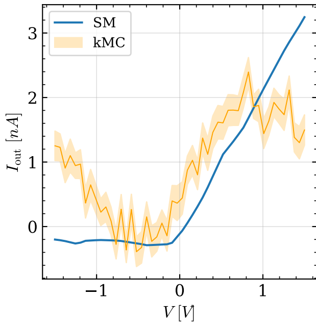
ReLU
