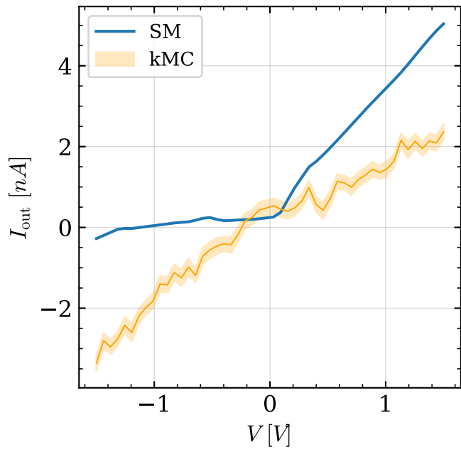
ReLU
