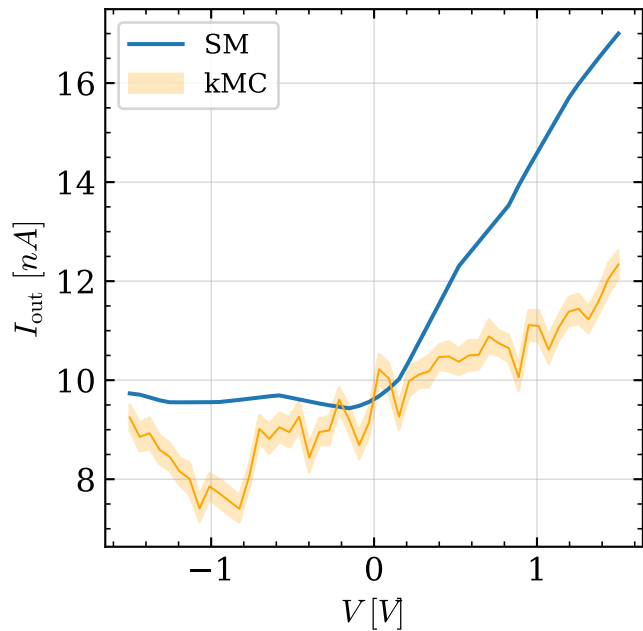
ReLU
