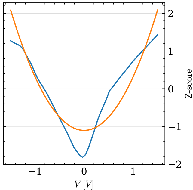
Z-scored target and solution
