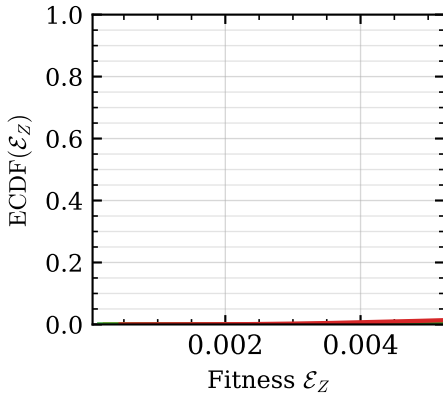
ReLU
