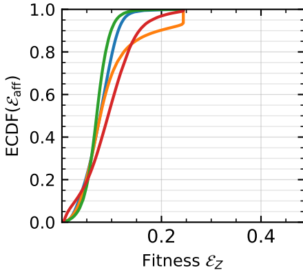
ReLU
