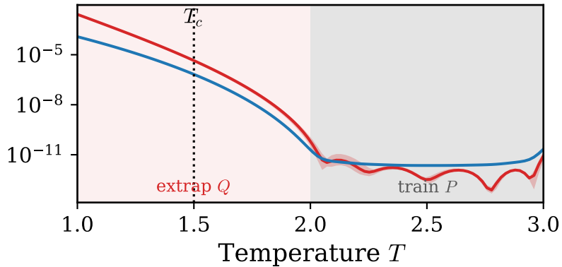
(a) Heisenberg
