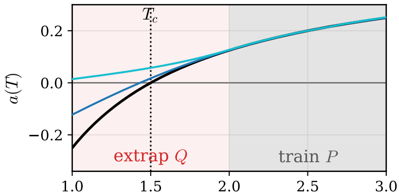
(a) Landau coefficient a(T)
