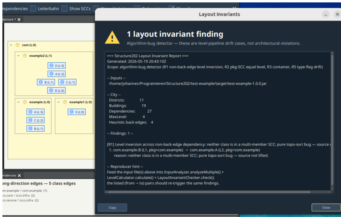
Figure 2: Implausibility alert in action. For this screenshot we deliberately injected a level-pipeline defect into LevelCalculator that misplaces class com.example.A on the wrong level (compare with Figure 1, left, which shows the correct placement of the same test JAR). The post-pipeline invariant checker catches the inconsistency immediately and pops up the Layout Invariants dialog: a single R1 finding with a copy-paste reproducer block tells the developer that the dependency B → A now runs against the computed levels. The status bar additionally reports the four wrong-direction class edges induced by the bug. No human inspection of the picture was needed to surface the defect; the alert is generated automatically by the consistency checks that run after every analysis.
