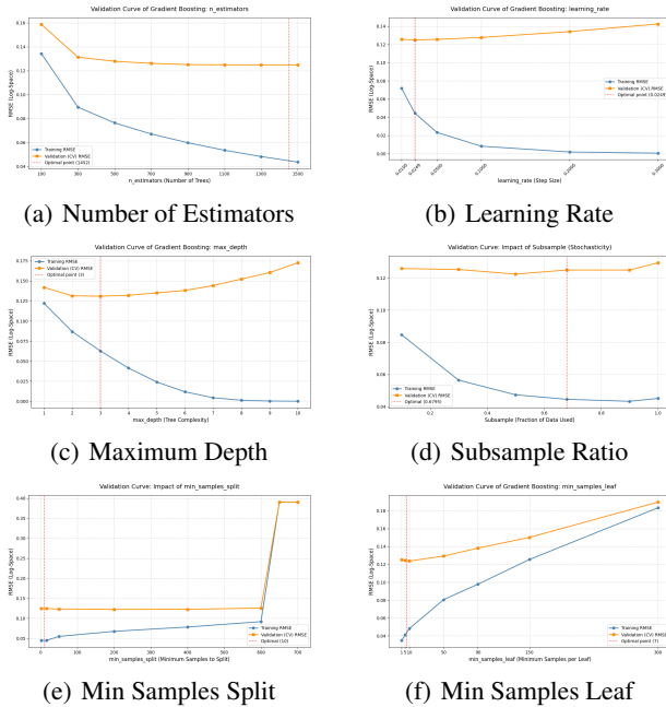
Figure 6. Validation curves for the six key hyperparameters of the Gradient Boosting Regressor. The blue line represents the Training RMSE, while the orange line indicates the Validation (CV) RMSE. Vertical dotted lines mark the optimal parameters identified by the tuning process.
