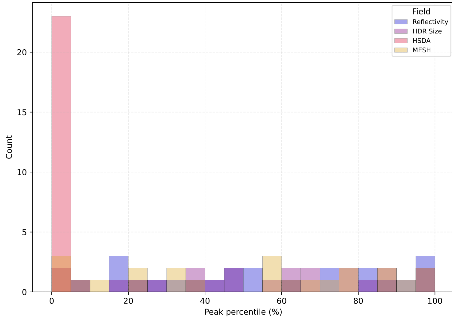
Histogram of Date-Peak Percentiles (Sig-severe)
