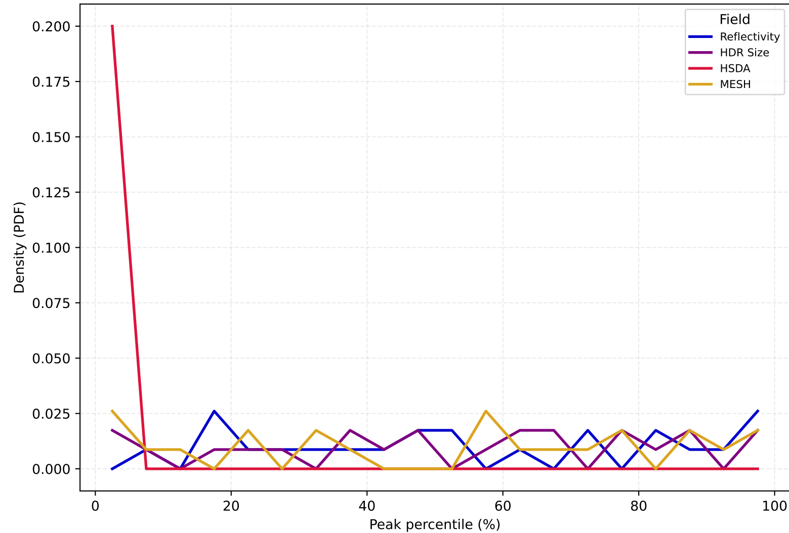
PDF of Date-Peak Percentiles (Sig-severe)
