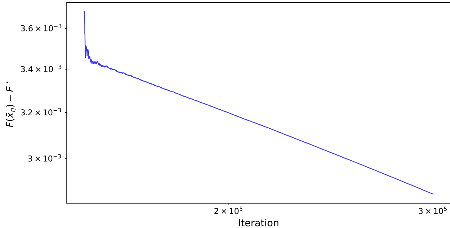
Convergence — Regime A ( c_2 = 0.2 , threshold < 0 )
