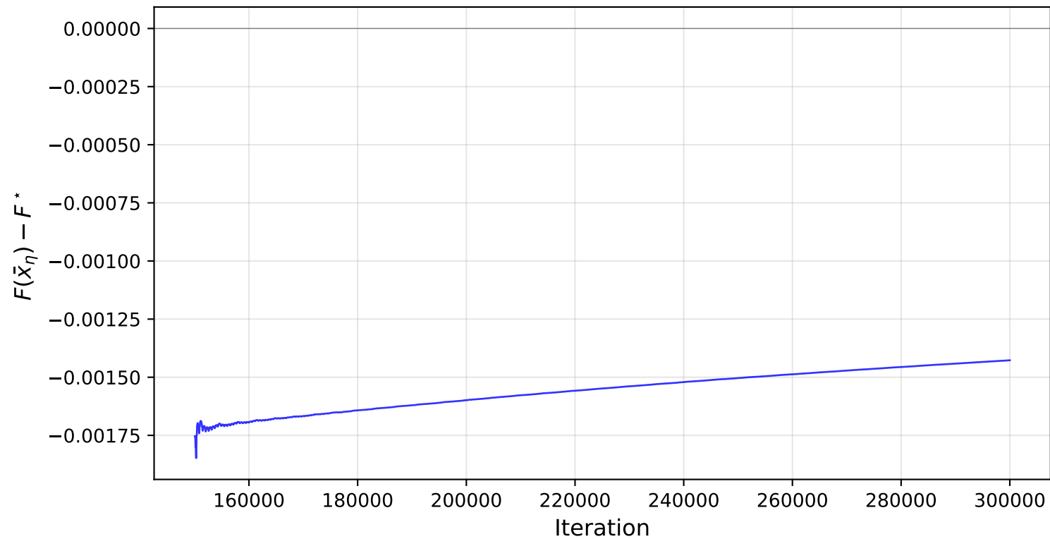
Convergence — Regime B ( c_2 = 0.30 , threshold > 0 )
