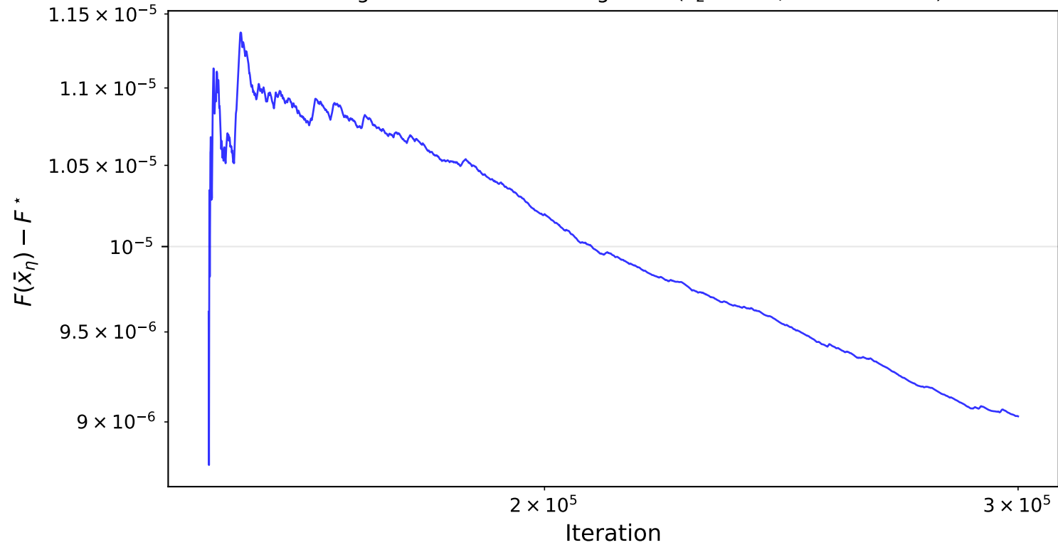
Convergence — Stochastic Regime A ( c_2 = 0.04 , threshold < 0 )
