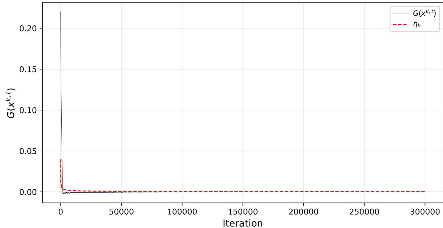
Feasibility — Stochastic Regime A ( c_2 = 0.04 , threshold < 0 )
