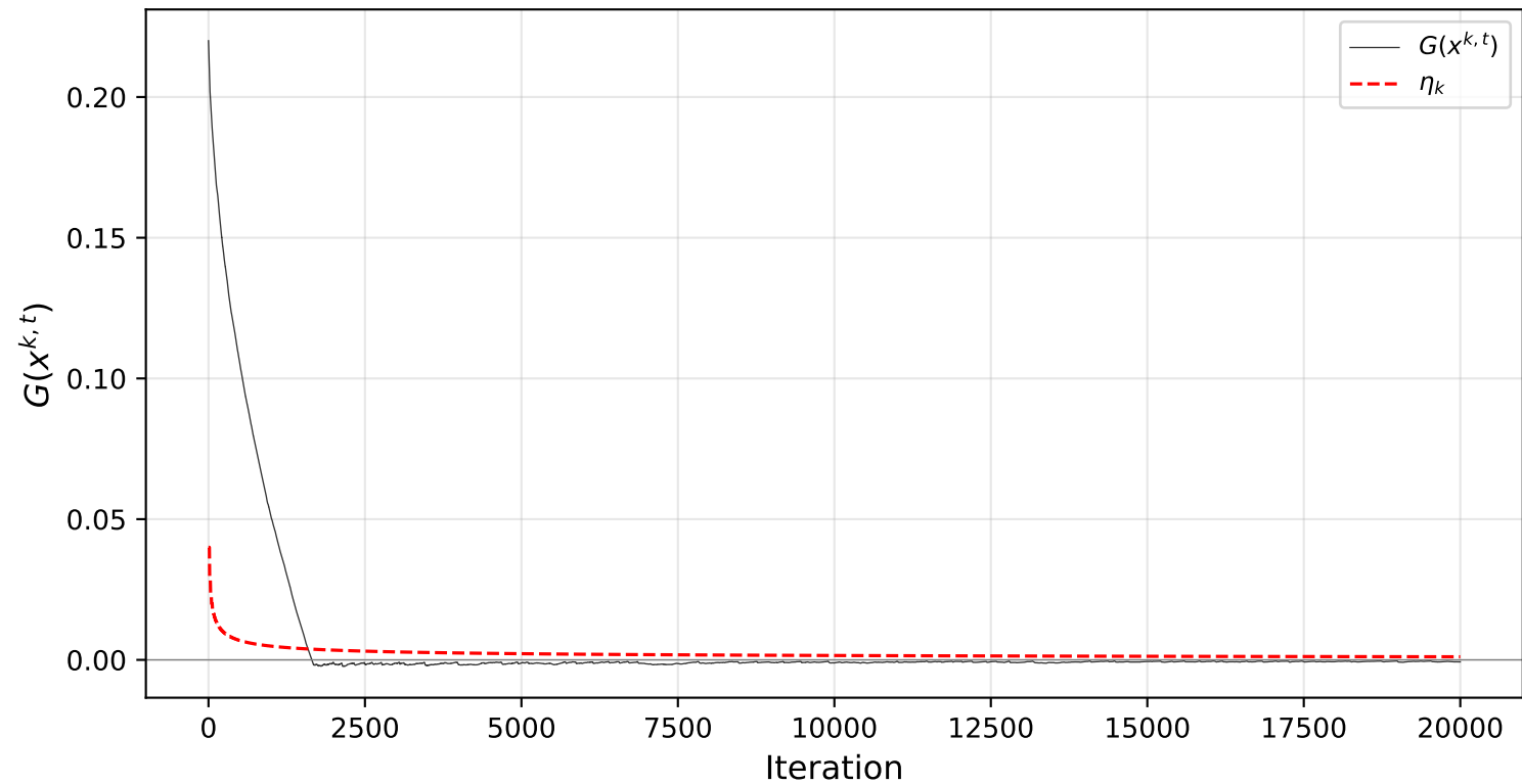
Feasibility (zoomed) — Stochastic Regime A ( c_2 = 0.04 , threshold < 0 )
