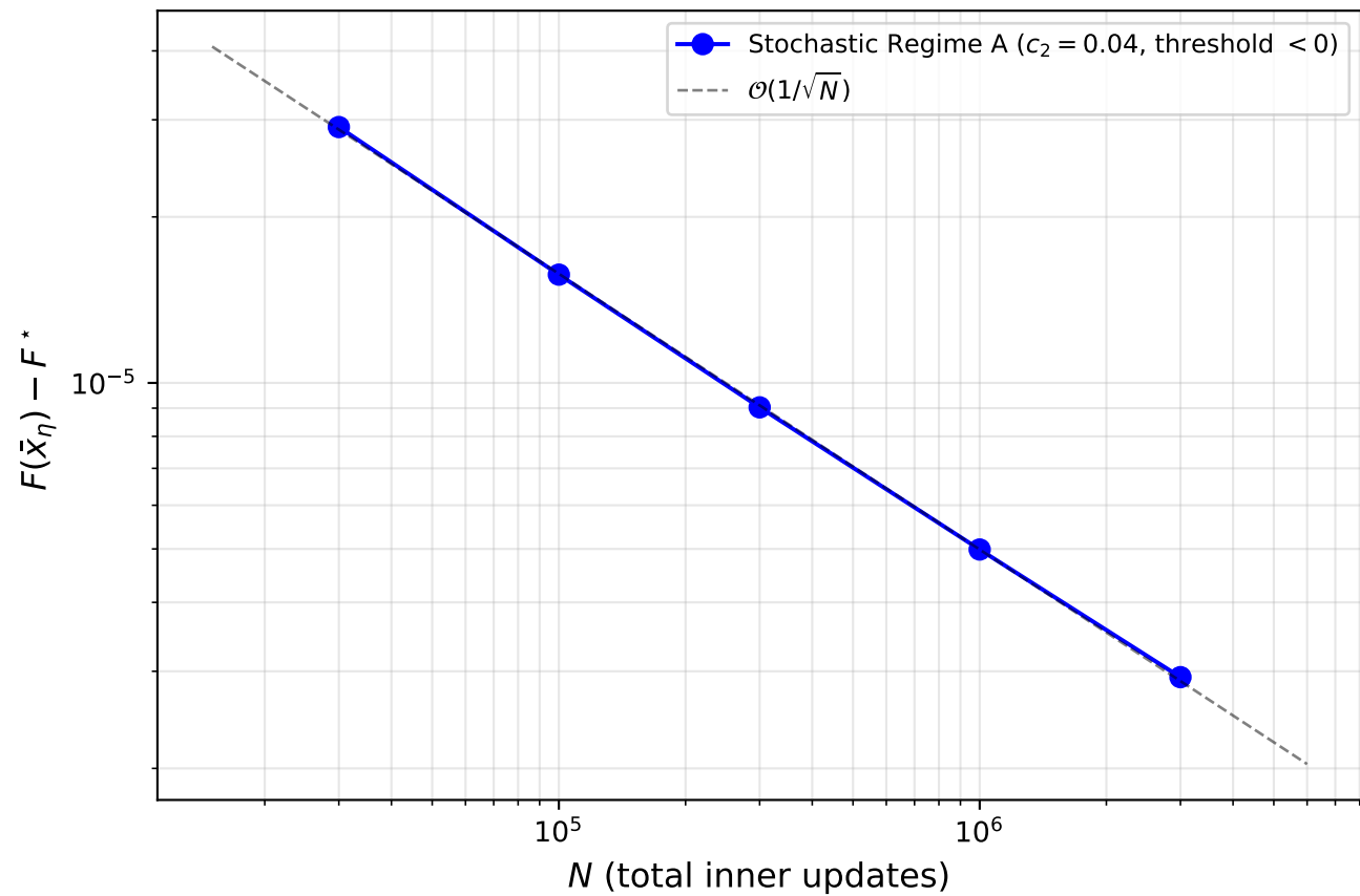
Rate — Stochastic Regime A ( c_2 = 0.04 , threshold < 0 )
