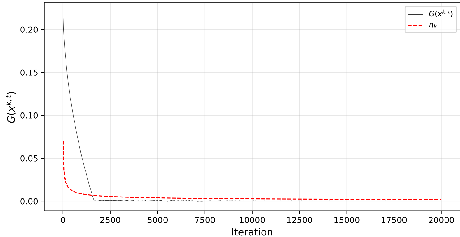
Feasibility (zoomed) — Stochastic Regime B ( c_2 = 0.07 , threshold > 0 )
