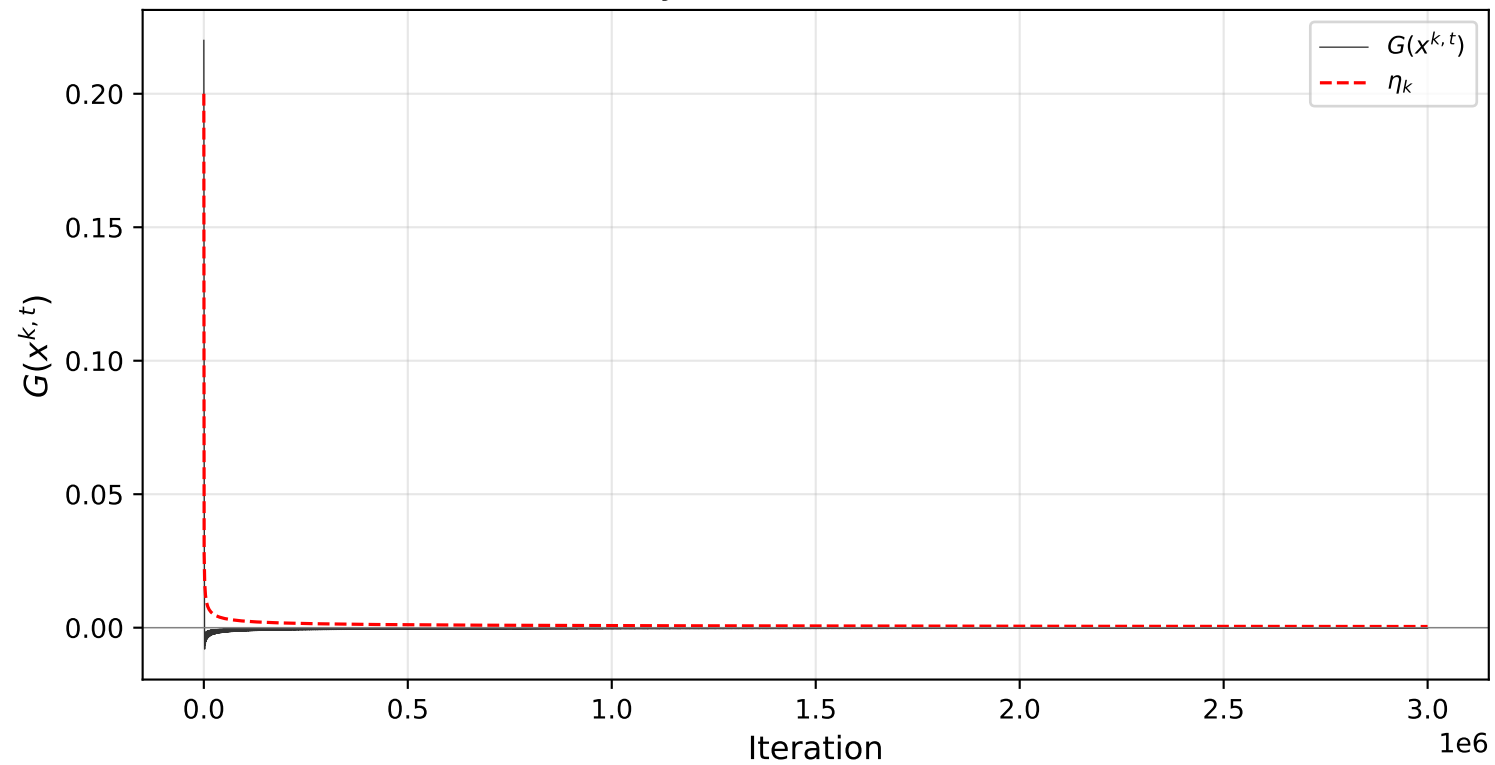
Feasibility — T = 15, N = 3,000,000
