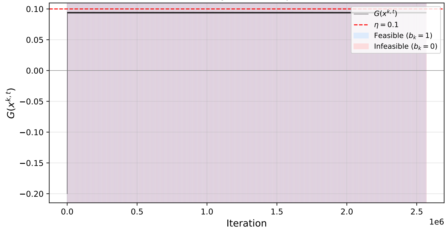
Feasibility — T = 15, \eta = 0.1
