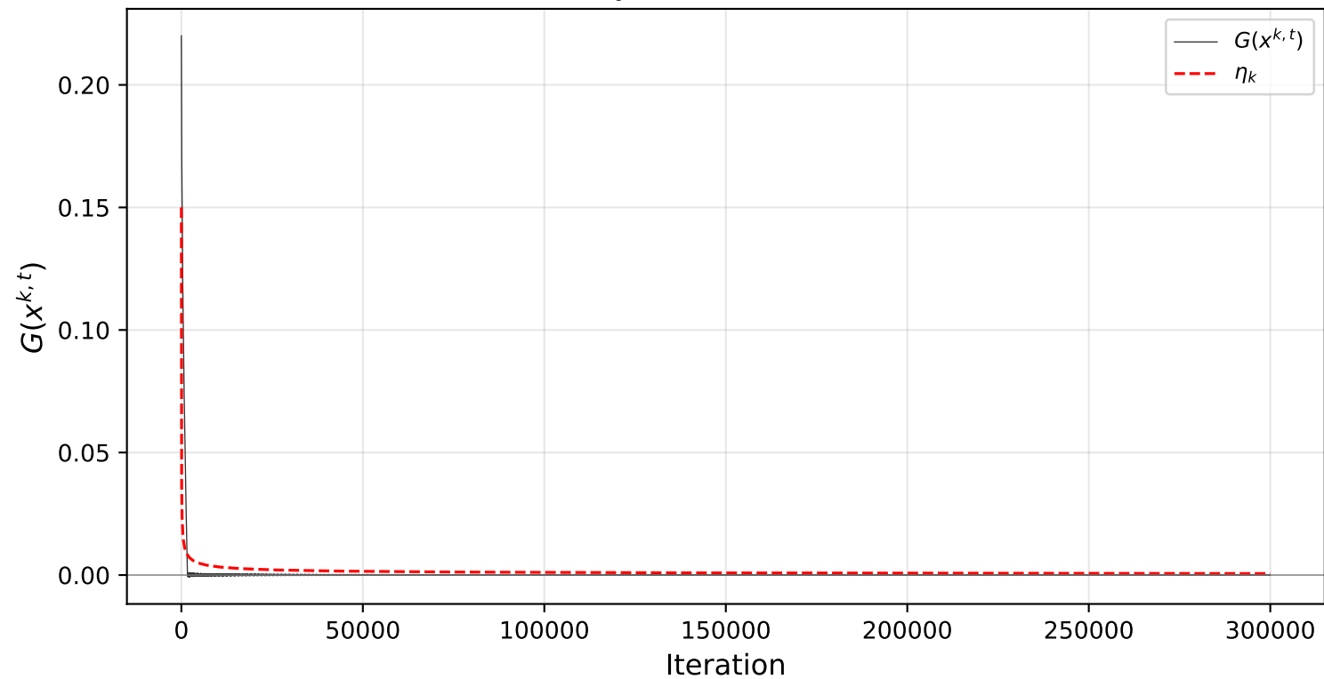
Feasibility — T = 5, N = 300,000
