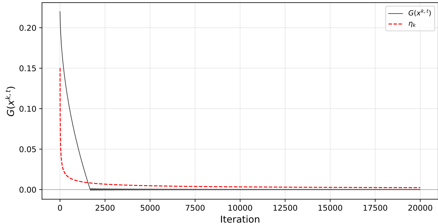
Feasibility (zoomed) — T = 5 , N = 300,000
