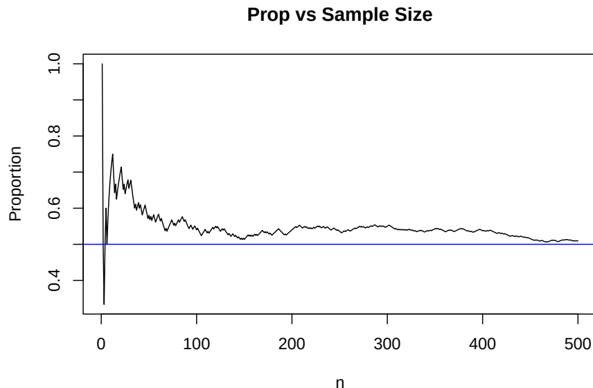
Figure 11.1: LLN Example with Coin Flips
