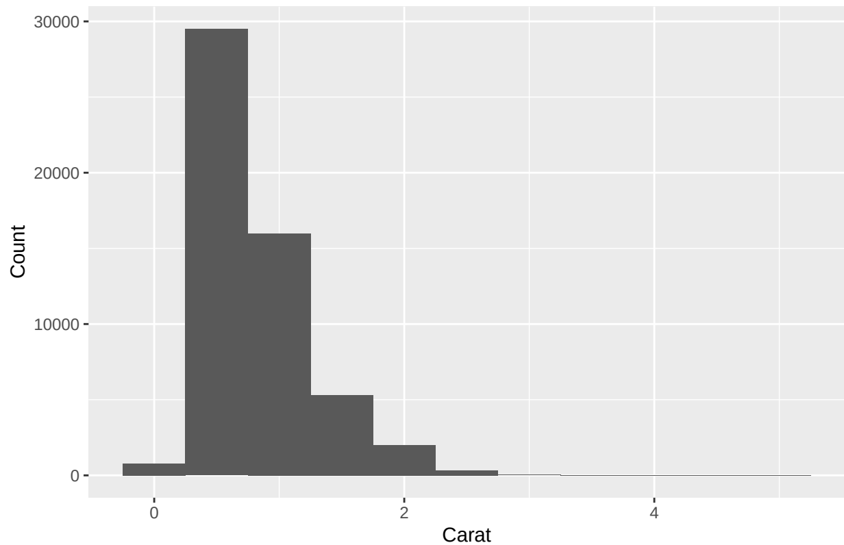
Histogram of Diamond Carats
