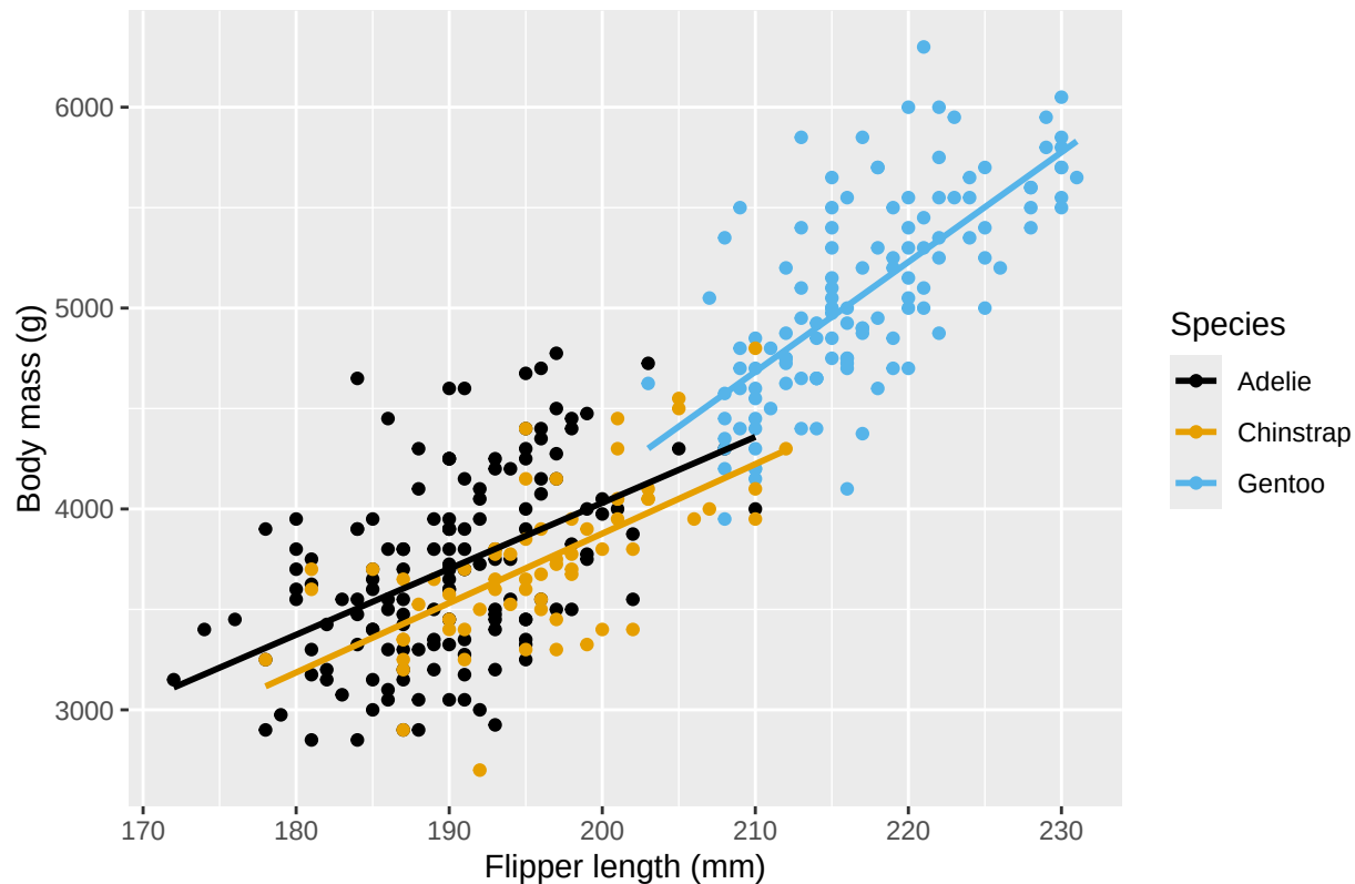
Body Mass and Flipper Length of Penguins
