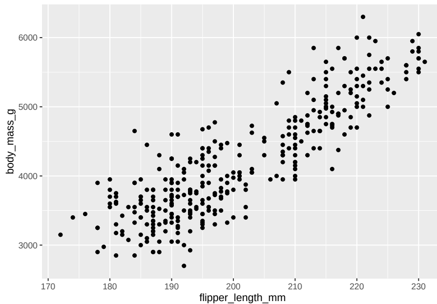
Figure 8.1: ( #fig:ch8scatter_plain ) Basic Scatterplot using ggplot
