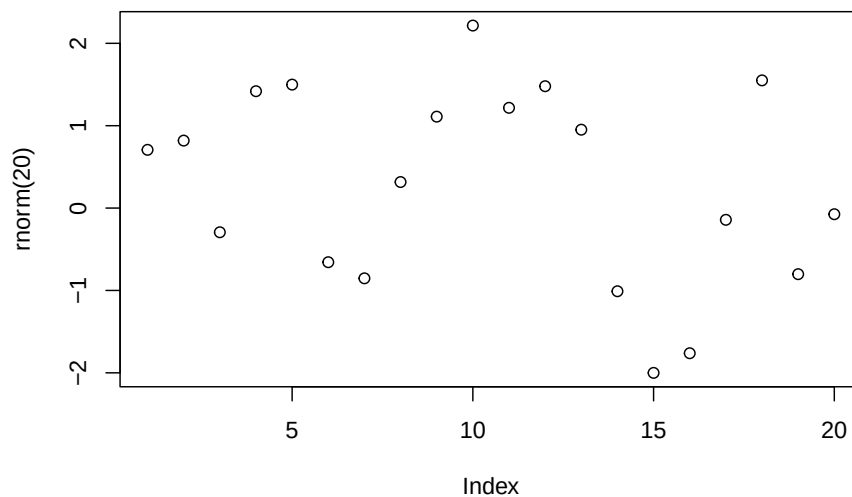
Figure 8.18: Visualization Simulations with Base R
