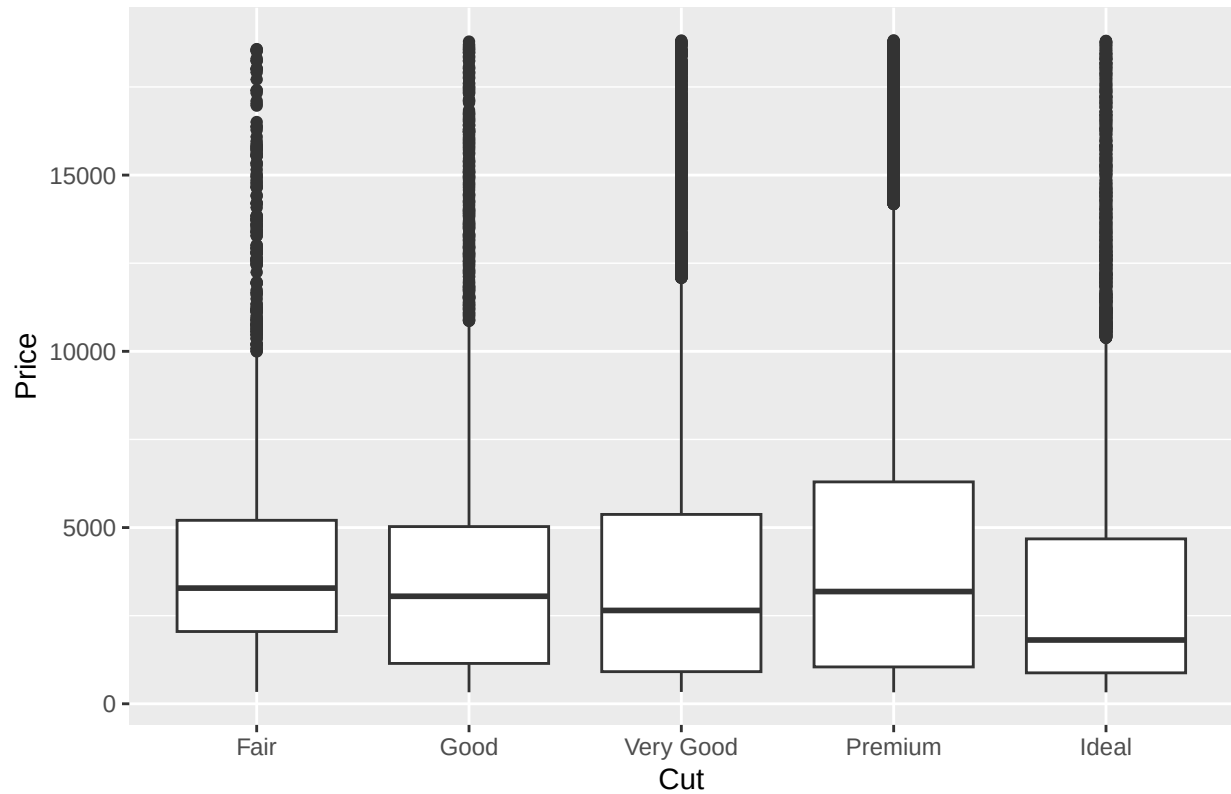
Boxplot of Prices across Cut
