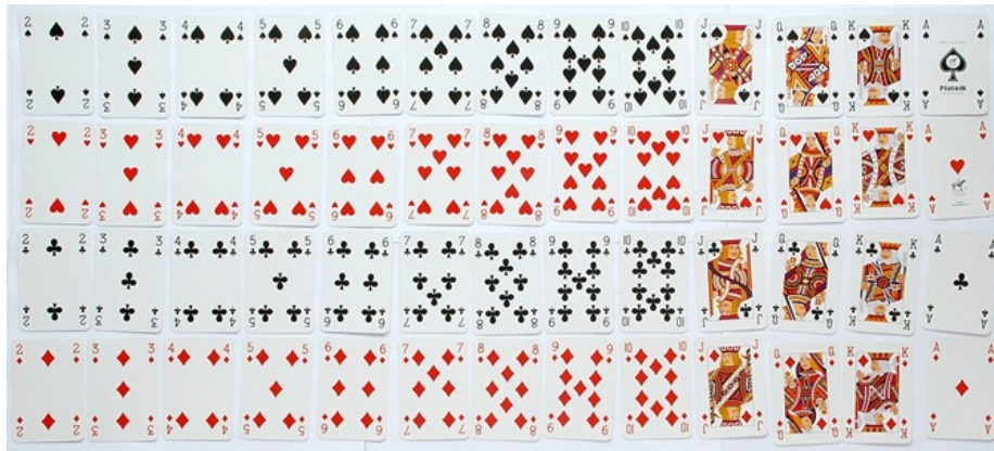
Figure 10.2: Sample Space of Drawing One Card from Standard Deck. Picture from wikipedia
