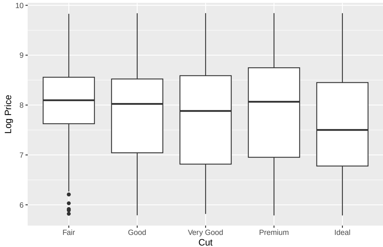
Boxplot of Log Prices across Cut
