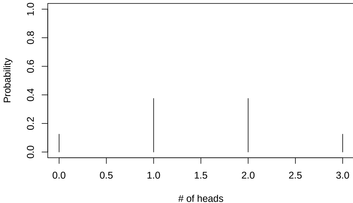
PMF for X
