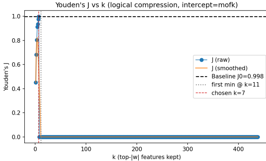
Figure 14. J versus retained rule size k for anytime compression. The curve provides a direct complexity-performance trade-off for selecting a deployable m -of- k rule. Note that the Youden’s- J falls off to zero after k=7 because the algorithm exits early if it reaches a Youden’s J -Index value of 1.0. See Figure 13 for an example of a real world dataset in which this is not the case.
