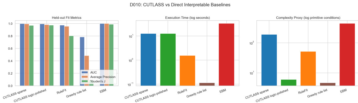
Figure 12. Direct interpretable-model summary on synthetic Case 1. EBM gives the strongest raw fit, but the CUTLASS logic-polished model achieves competitive discrimination with far lower complexity than EBM and materially stronger fidelity than RuleFit or the greedy rule list.
