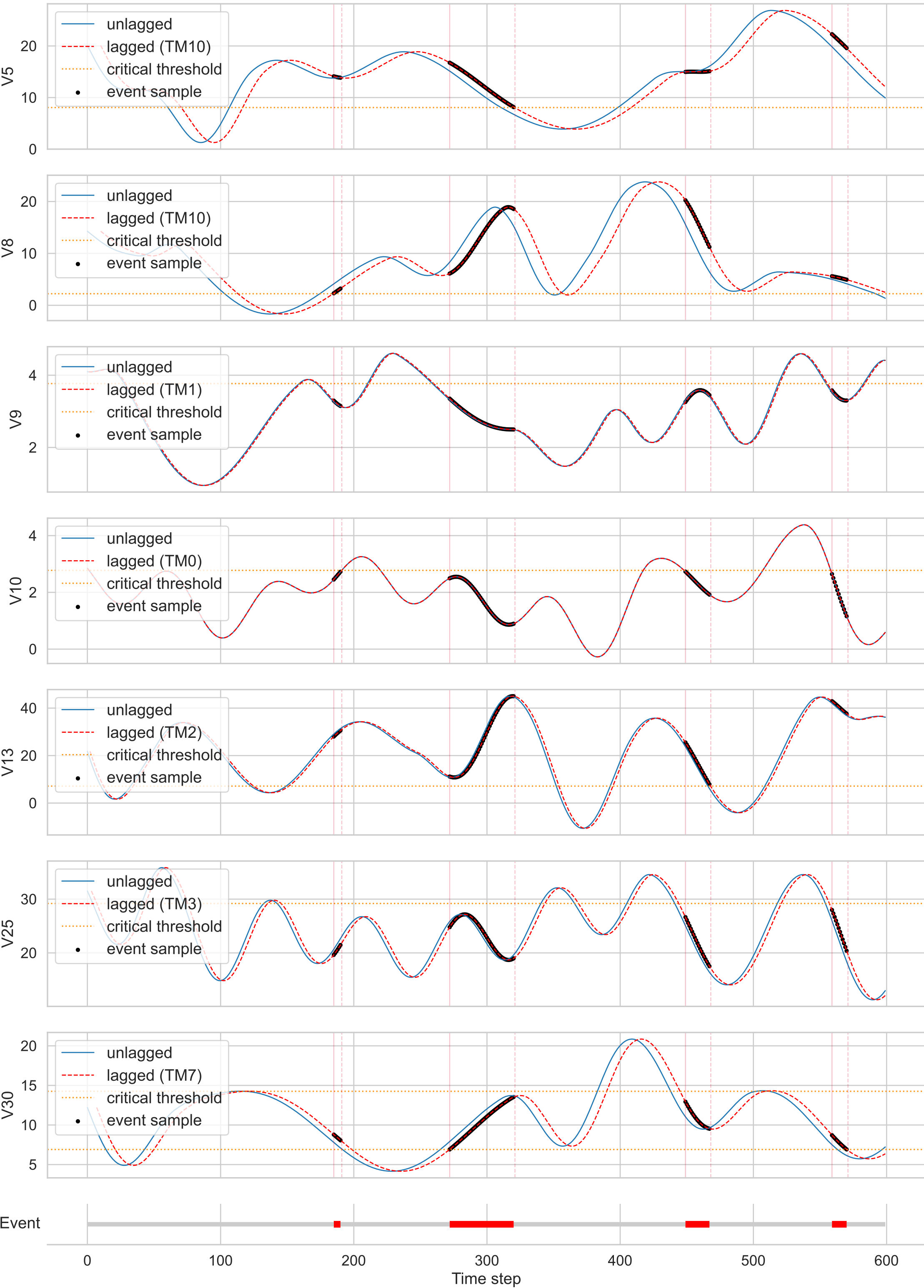
Relevant sensor curves with lagged overlays, critical thresholds, event boundaries, and timeline indicator (first 600 timesteps)
