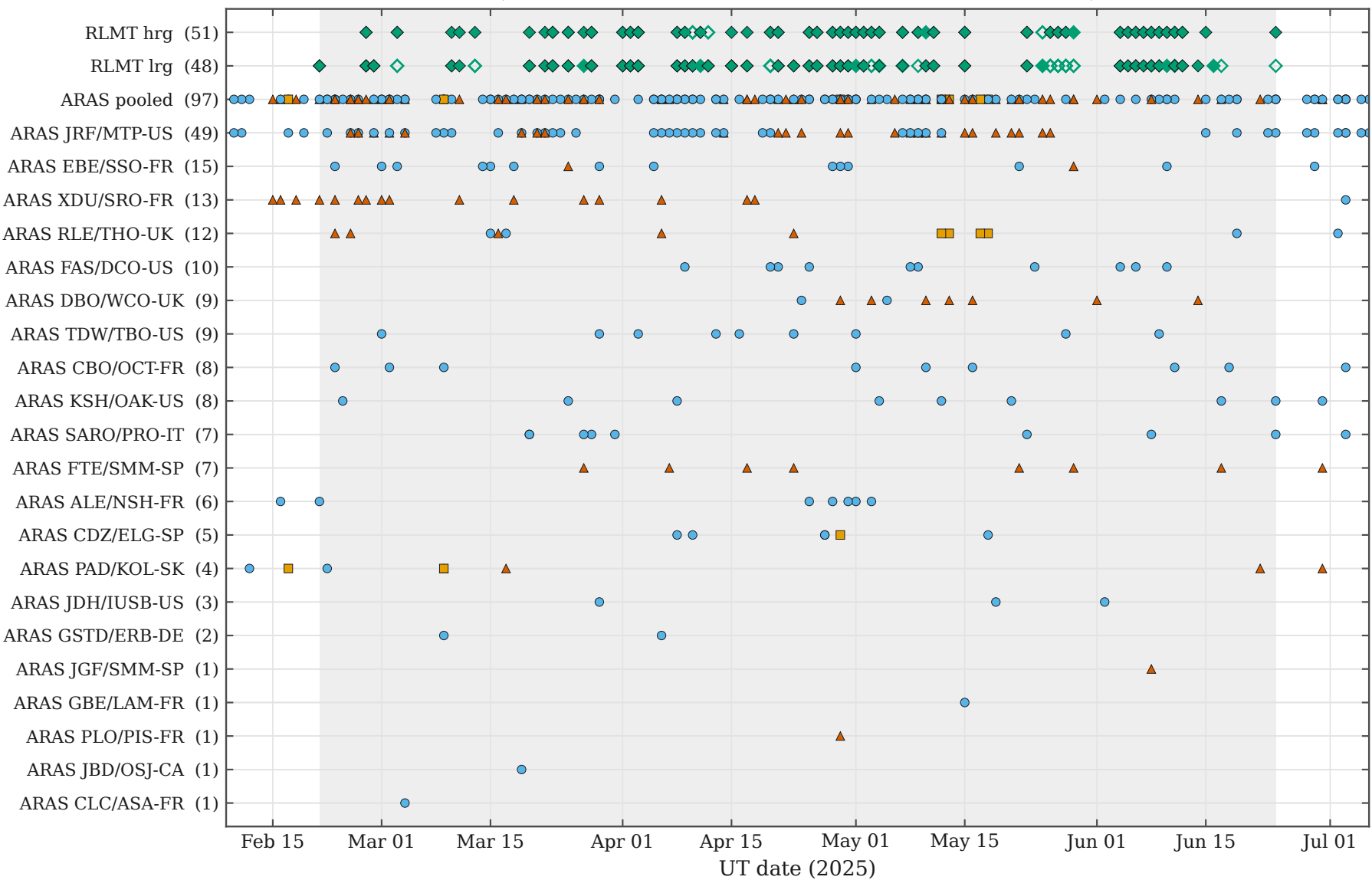
Who took an H \alpha spectrum of T CrB on which night (in brackets: dates inside the shaded RLMT window)
