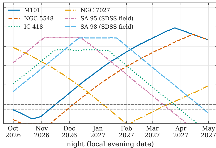
Galaxies and calibrators
