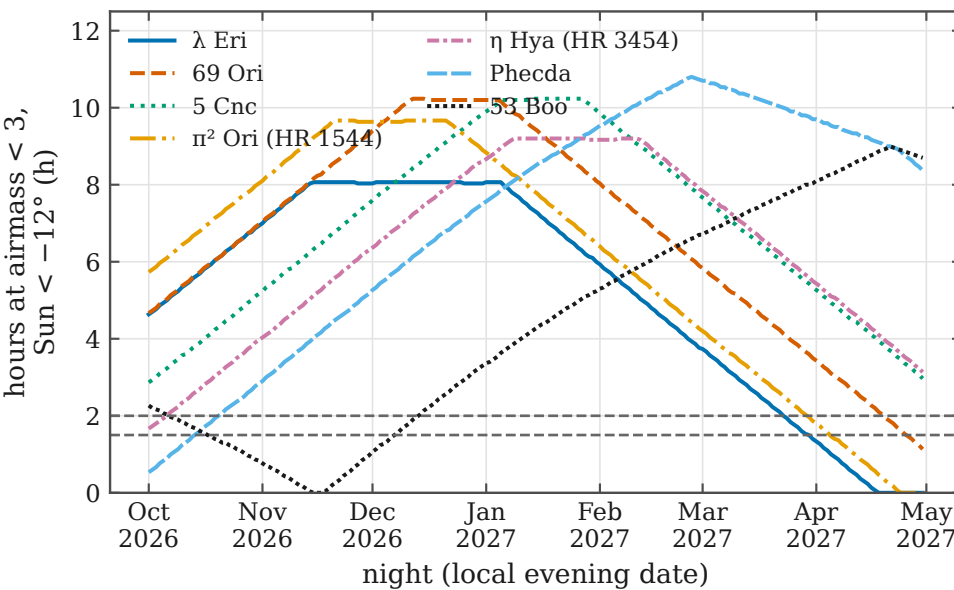
Be stars and autumn standards
