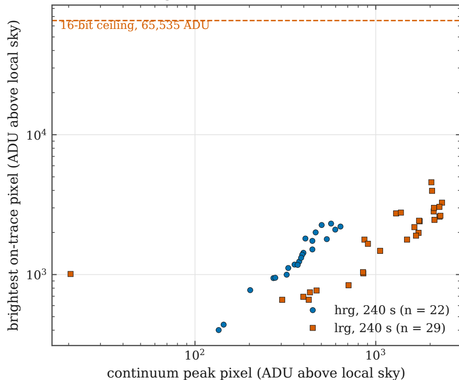
T CrB, 2025 grism frames (ASI): far below the clip
