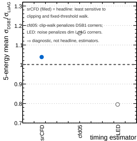
C estimator dependence
