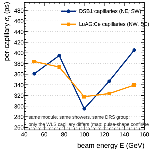
A same-shower timing widths (srCFI)
