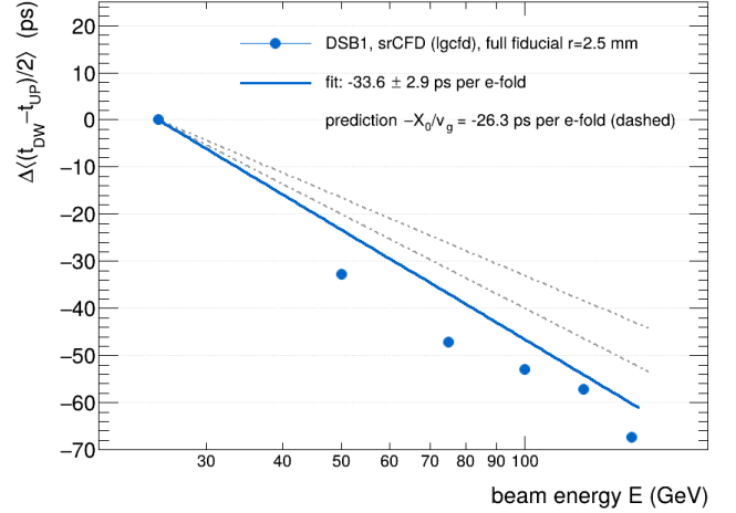
Figure 8: Energy dependence of the mean dual-end timing asymmetry \Delta((t_{\text{DW}} - t_{\text{UP}})/2) (DSB1, srCFD, full fiducial), relative to 25 GeV. The dashed band is the -X_0/v_g expectation from shower-maximum migration. The fitted slope is -33.6 \pm 2.9 ps per e -fold (acceptance-conditional; see text).
