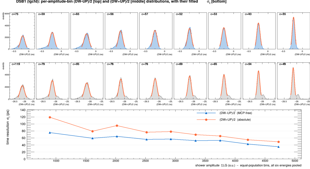
Figure 4: DSB1 timing distributions, all energies pooled and binned by amplitude \Sigma LG . Top: (DW - UP)/2 (MCP-free). Middle: (DW + UP)/2 (absolute). Each \sigma (ps) is the central-peak Gaussian fit. Bottom: the fitted \sigma_t versus amplitude for both estimators.
