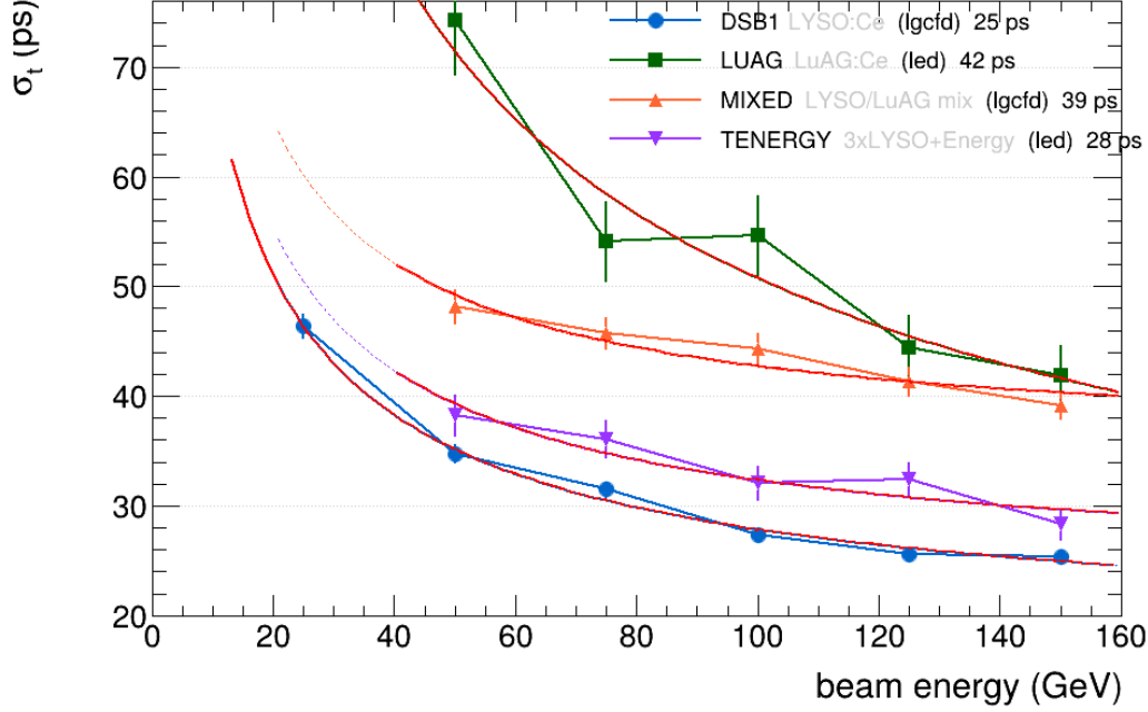
Figure 7: Best-achievable (DW - UP)/2 resolution versus energy for the four builds. The ordering follows the scintillation light yield: high-light LYSO (DSB1) lowest, low-light LuAG highest.
