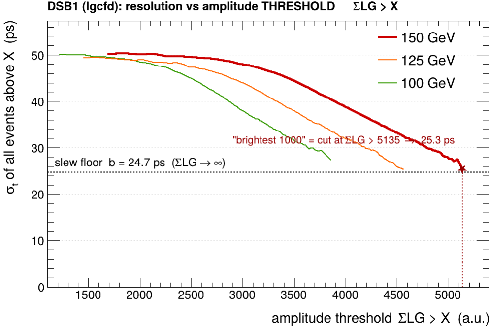
Figure 6: DSB1 resolution versus amplitude threshold: \sigma_t of all events with \Sigma LG > X , per energy. Raising the cut keeps brighter showers and the resolution approaches the floor. The “brightest 1000” headline is the single point at \Sigma LG > 5135 (★).
