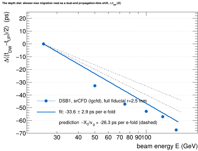
Figure 8: Energy dependence of the mean dual-end timing asymmetry \Delta((t_{\text{DW}} - t_{\text{UP}})/2) (DSB1, srCFD, full fiducial), relative to 25 GeV. The dashed band is the -X_0/v_g expectation from shower-maximum migration. The fitted slope is -33.6 \pm 2.9 ps per e -fold (acceptance-conditional; see text).
