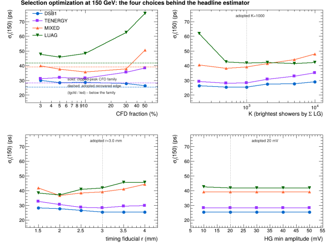
Figure A.9: Selection optimization at 150 GeV for all four builds: (a) timing source as a function of CFD fraction on the clipped peak (solid) with the adopted recovered-edge source overlaid (dashed); (b) resolution versus the brightest- N selection K ; (c) versus timing fiducial radius; (d) versus the per-channel HG threshold. Dashed grey lines mark the adopted working points.
