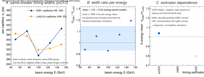
Figure 7: Same-shower comparison in the MIXED module (corner map confirmed by pulse-shape discriminants). Left: per-capillary timing widths versus energy for the DSB1 (NE, SW) and LuAG:Ce (NW, SE) capillary pairs under srCFD; widths are same-layer in-event pair differences divided by \sqrt{2} , so common-mode terms cancel. Centre: the width ratio per energy with the \pm 1 RMS energy-scatter band; the scatter dominates the statistical uncertainty. Right: estimator dependence (srCFD headline; cfd05 and LED diagnostic).
