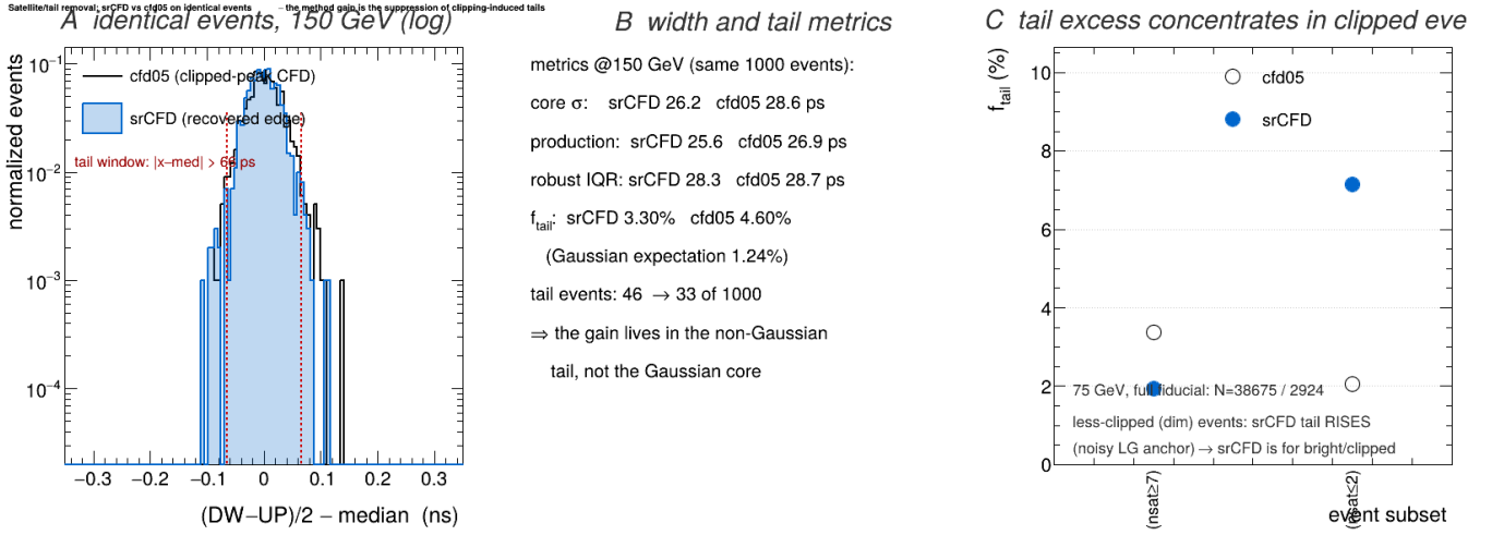
Figure B.11: Tail suppression by the saturation-recovered CFD on identical events (DSB1, brightest-1000, production selection). (A) The per-event (\text{DW} - \text{UP})/2 distribution at 150 GeV under cfd05 (line) and srCFD (filled), median-centred, unit-normalized, logarithmic scale; the common tail window |x - \text{med}| > 66 \text{ ps} ( 2.5\sigma of the srCFD core) is marked. (B) Width and tail metrics on the same events: the production widths are 25.6 (srCFD) vs 26.9 ps (cfd05) while the tail fraction drops from 4.60% to 3.30% (Gaussian expectation 1.24%; the srCFD remainder reflects genuine shower tails). (C) At 75 GeV (full-fiducial sample; in the brightest-1000 the less-clipped subset is empty), the cfd05 tail excess concentrates in the clipped subset, while on dim unclipped pulses srCFD's low-gain anchor is noisy and its tail rises — each estimator is biased outside its design regime, the basis of the per-regime source rule.
