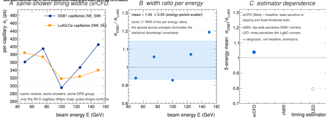
Figure 7: Same-shower comparison in the MIXED module (corner map confirmed by pulse-shape discriminants). Left: per-capillary timing widths versus energy for the DSB1 (NE, SW) and LuAG:Ce (NW, SE) capillary pairs under srCFD; widths are same-layer in-event pair differences divided by \sqrt{2} , so common-mode terms cancel. Centre: the width ratio per energy with the \pm 1 RMS energy-scatter band; the scatter dominates the statistical uncertainty. Right: estimator dependence (srCFD headline; cdf05 and LED diagnostic).
