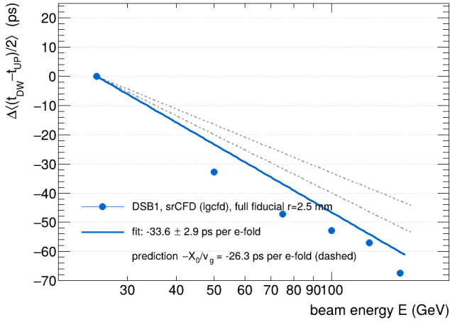
The depth dial: shower-max migration read as a dual-end propagation-time shift, \Delta(t_{\text{DW}} - t_{\text{UP}})/2 (E)
