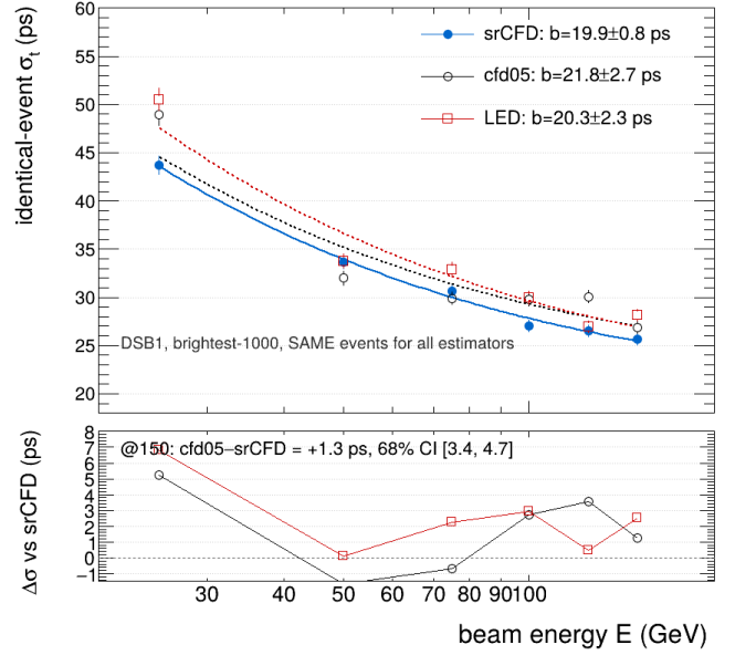
Method gain, post-fix: saturation-recovered CFD vs clipped-peak CFD and LED on identical events (DSB1)
