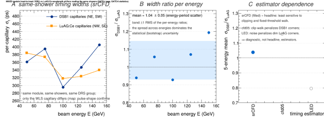
Figure 8: Same-shower comparison in the MIXED module (corner map confirmed by pulse-shape discriminants). Left: per-capillary timing widths versus energy for the DSB1 (NE, SW) and LuAG:Ce (NW, SE) capillary pairs under srCFD; widths are same-layer in-event pair differences divided by \sqrt{2} , so common-mode terms cancel. Centre: the width ratio per energy with the \pm 1 RMS energy-scatter band; the scatter dominates the statistical uncertainty. Right: estimator dependence (srCFD headline; cfdf05 and LED diagnostic).
