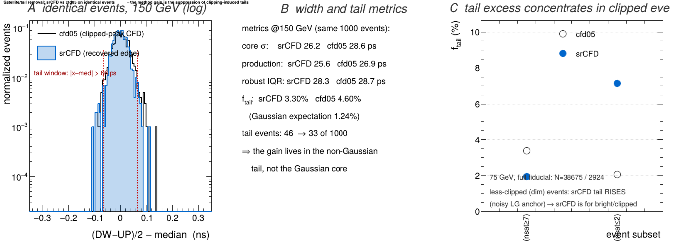
Figure 6: Tail suppression by the saturation-recovered CFD on identical events (DSB1, brightest-1000, production selection). (A) The per-event (\text{DW} - \text{UP})/2 distribution at 150 GeV under cfd05 (line) and srCFD (filled), median-centred, unit-normalized, logarithmic scale; the common tail window |x - \text{med}| > 66 ps ( 2.5\sigma of the srCFD core) is marked. (B) Width and tail metrics on the same events: the production widths are 25.6 (srCFD) vs 26.9 ps (cfd05) while the tail fraction drops from 4.60% to 3.30% (Gaussian expectation 1.24%; the srCFD remainder reflects genuine shower tails). (C) At 75 GeV (full-fiducial sample; in the brightest-1000 the less-clipped subset is empty), the cfd05 tail excess concentrates in the clipped subset, while on dim unclipped pulses srCFD’s low-gain anchor is noisy and its tail rises — each estimator is biased outside its design regime, the basis of the per-regime source rule.
