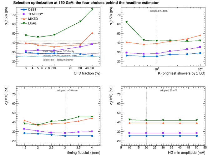
Figure A.10: Selection optimization at 150 GeV for all four builds: (a) timing source as a function of CFD fraction on the clipped peak (solid) with the adopted recovered-edge source overlaid (dashed); (b) resolution versus the brightest-N selection K; (c) versus timing fiducial radius; (d) versus the per-channel HG threshold. Dashed grey lines mark the adopted working points.
