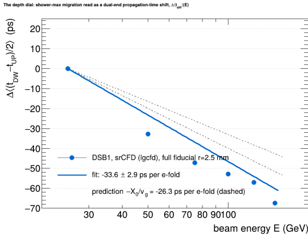
Figure 9: Energy dependence of the mean dual-end timing asymmetry \Delta((t_{\text{DW}} - t_{\text{UP}})/2) (DSB1, srCFD, full fiducial), relative to 25 GeV. The dashed band is the -X_0/v_g expectation from shower-maximum migration. The fitted slope is -33.6 \pm 2.9 ps per e-fold (acceptance-conditional; see text).
