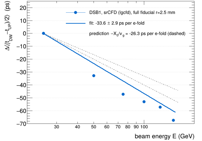
Figure 9: Energy dependence of the mean dual-end timing asymmetry \Delta((t_{\text{DW}} - t_{\text{UP}})/2) (DSB1, srCFD, full fiducial), relative to 25 GeV. The dashed band is the -X_0/v_g expectation from shower-maximum migration. The fitted slope is -33.6 \pm 2.9 ps per e -fold (acceptance-conditional; see text).
