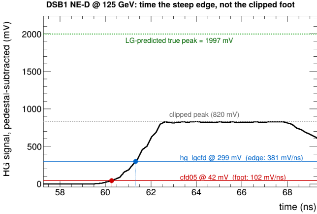
Figure 4: A single saturated high-gain waveform (125 GeV). The recorded pulse clips at 820 mV (grey); the low-gain copy predicts a true peak of 1997 mV (green). The CFD at 15% of the predicted peak (hg_lgcfd, blue) times an edge of 381 mV/ns, against 102 mV/ns at the clipped-peak foot where the 5% CFD (cfd05, red) must sit — a factor 3.7 steeper.
