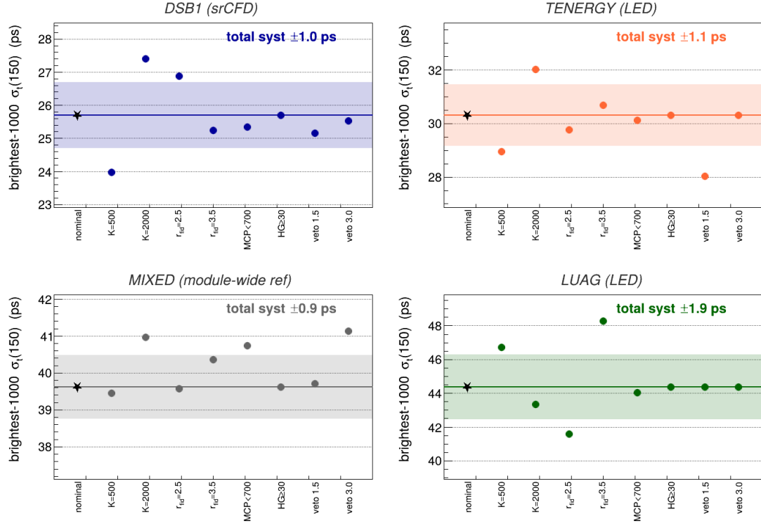
Figure A.10: Systematic stability of the brightest-1000 \sigma_t(150) for each build under the production estimator chain: the nominal value (star) with the total-systematic (RMS) band of Table 2, and each selection variation of Table 2 as a point, including the in-event veto-window variations. The annotated total is the RMS of the shifts; authoritative values are those of Table 2 (floors: Table 1). The largest excursions are the brightness-selection variations ( K ).
