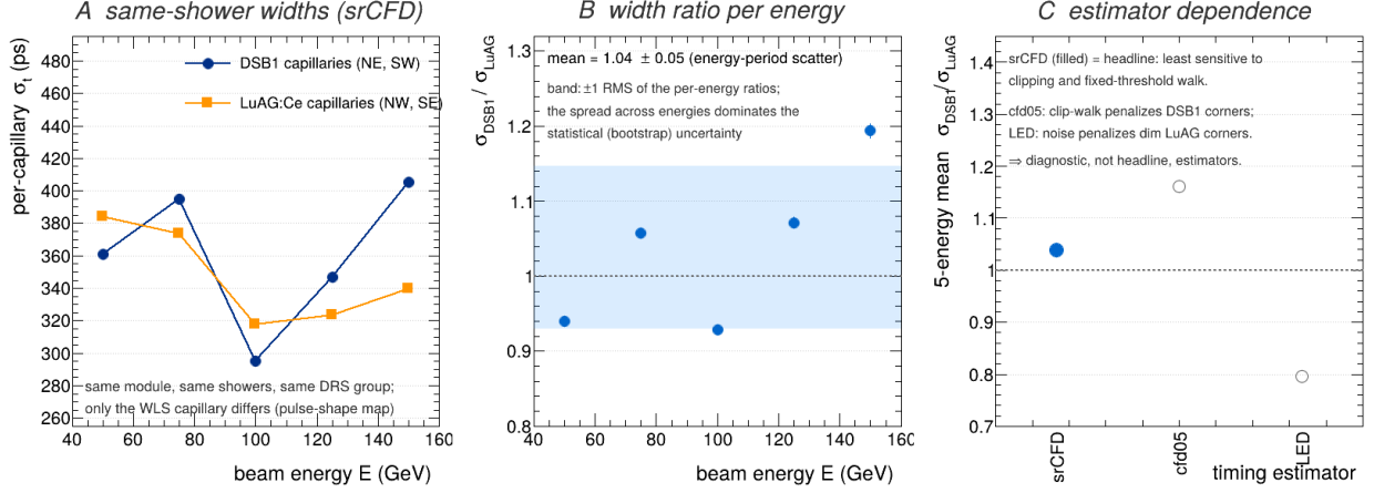
Figure 7: Same-shower comparison in the MIXED module (corner map confirmed by pulse-shape discriminants). (A) Per-capillary timing widths versus energy for the DSB1 (NE, SW) and LuAG:Ce (NW, SE) capillary pairs under srCFD; widths are same-layer in-event pair differences divided by \sqrt{2} , so common-mode terms cancel. (B) The width ratio per energy with the \pm 1 RMS energy-scatter band; the scatter dominates the statistical uncertainty. (C) Estimator dependence (srCFD headline; cfd05 and LED diagnostic).
