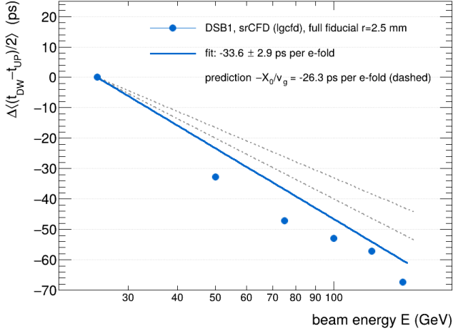
Figure 8: Energy dependence of the mean dual-end timing asymmetry \Delta((t_{\text{DW}} - t_{\text{UP}})/2) (DSB1, srCFD, full fiducial), relative to 25 GeV. The dashed band is the -X_0/v_g expectation from shower-maximum migration. The fitted slope is -33.6 \pm 2.9 ps per e -fold (acceptance-conditional; see text).
