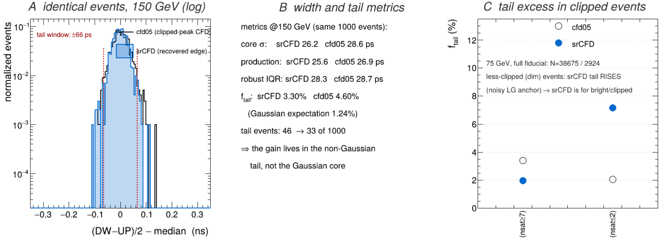
Figure B.12: Tail suppression by the saturation-recovered CFD on identical events (DSB1, brightest-1000, production selection). (A) The per-event (\text{DW} - \text{UP})/2 distribution at 150 GeV under cfd05 (line) and srCFD (filled), median-centred, unit-normalized, logarithmic scale; the common tail window |x - \text{med}| > 66 ps ( 2.5\sigma of the srCFD core) is marked. (B) Width and tail metrics on the same events: the production widths are 25.6 (srCFD) vs 26.9 ps (cfd05) while the tail fraction drops from 4.60% to 3.30% (Gaussian expectation 1.24%; the srCFD remainder reflects genuine shower tails). (C) At 75 GeV (full-fiducial sample; in the brightest-1000 the less-clipped subset is empty), the cfd05 tail excess concentrates in the clipped subset, while on dim unclipped pulses srCFD's low-gain anchor is noisy and its tail rises — each estimator is biased outside its design regime, the basis of the per-regime source rule.
