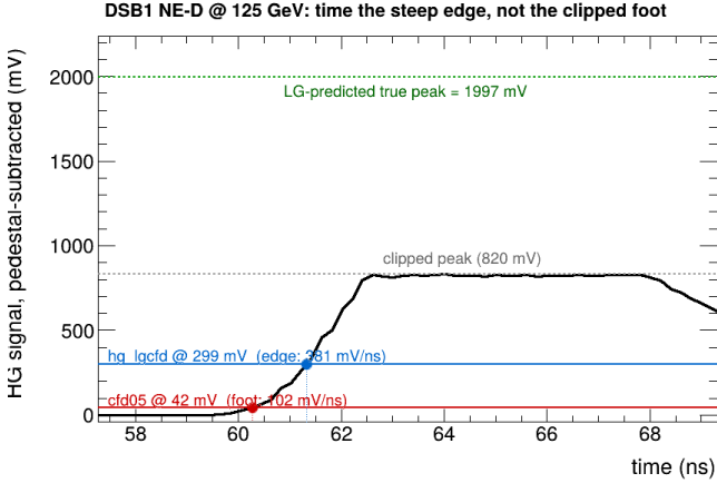
Figure 4: A single saturated high-gain waveform (125 GeV). The recorded pulse clips at 820 mV (grey); the low-gain copy predicts a true peak of 1997 mV (green). The CFDF at 15% of the predicted peak (hg_lgcfd, blue) times an edge of 381 mV/ns, against 102 mV/ns at the clipped-peak foot where the 5% CFDF (cfd05, red) must sit — a factor 3.7 steeper.
