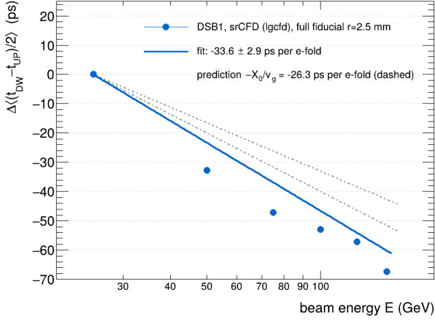
Figure 9: Energy dependence of the mean dual-end timing asymmetry \Delta((t_{\text{DW}} - t_{\text{UP}})/2) (DSB1, srCFD, full fiducial), relative to 25 GeV. The dashed band is the -X_0/v_g expectation from shower-maximum migration. The fitted slope is -33.6 \pm 2.9 ps per e -fold (acceptance-conditional; see text).
