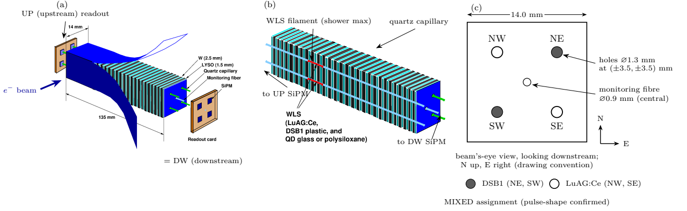
Figure 1: Schematic geometry used by the timing analysis (adapted from Ref. [1], the detailed apparatus reference). (a) The compact RADiCAL shower-maximum module: alternating tungsten absorber and LYSO:Ce scintillator plates, traversed by quartz capillaries read out by SiPMs at both the upstream (UP) and downstream (DW) faces; the timing observable of this paper is built from the difference of the two ends (Sec. 4). (b) The wavelength-shifting readout concept: a short WLS filament positioned at shower-maximum depth inside each quartz capillary converts the local scintillation light and pipes it to both SiPMs. (c) Beam's-eye corner convention used throughout (looking downstream; N up, E right by drawing convention): four capillaries at (\pm 3.5, \pm 3.5) mm in the 14.0 \times 14.0 mm 2 cell. In the MIXED module the two materials occupy opposite diagonals — NE + SW = DSB1, NW + SE = LuAG:Ce — so the same event provides DSB1 and LuAG:Ce timing observables in a common module and beam exposure (Sec. 6). This material assignment is the pulse-shape-confirmed map used in the same-shower control; it is not inferred from this schematic.
