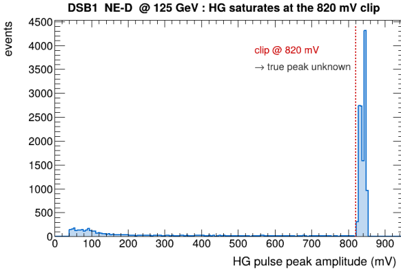
Figure 2: Distribution of recorded high-gain pulse-peak amplitudes (one channel, 125 GeV). The pile-up at \approx 820 mV is the digitiser clip: most showers saturate, so the true peak — and the steep edge that leads to it — is not directly recorded.
