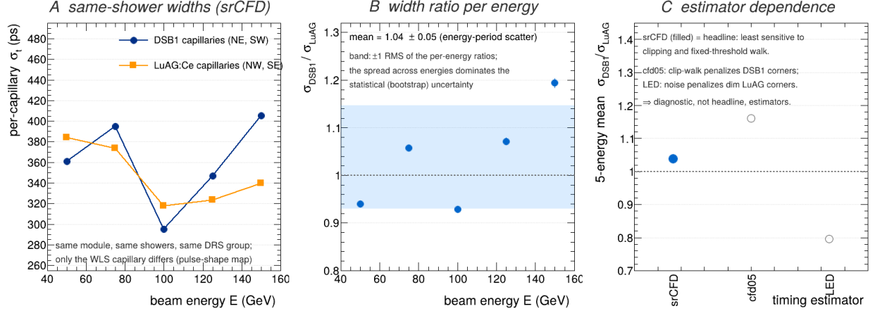
Figure 8: Same-shower comparison in the MIXED module (corner map confirmed by pulse-shape discriminants). (A) Per-capillary timing widths versus energy for the DSB1 (NE, SW) and LuAG:Ce (NW, SE) capillary pairs under srCFD; widths are same-layer in-event pair differences divided by \sqrt{2} , so common-mode terms cancel. (B) The width ratio per energy with the \pm 1 RMS energy-scatter band; the scatter dominates the statistical uncertainty. (C) Estimator dependence (srCFD headline; cfd05 and LED diagnostic).
